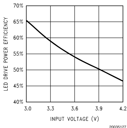
FIGURE 7. LM2750 LED Drive Efficiency. 6 LEDs, I_{LED} = 20mA each, V_{LED} = 4.0V
