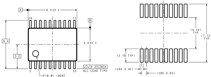
LAND PATTERN RECOMMENDATION
