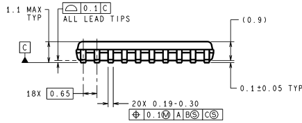
DIMENSIONS ARE IN MILLIMETERS
