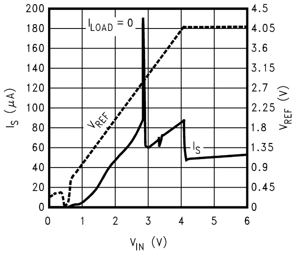
Power-Up Response (4.096V)
