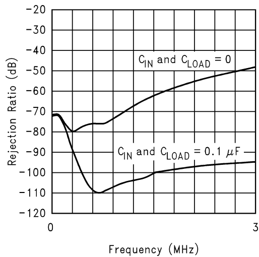
Power Supply Rejection Ratio
