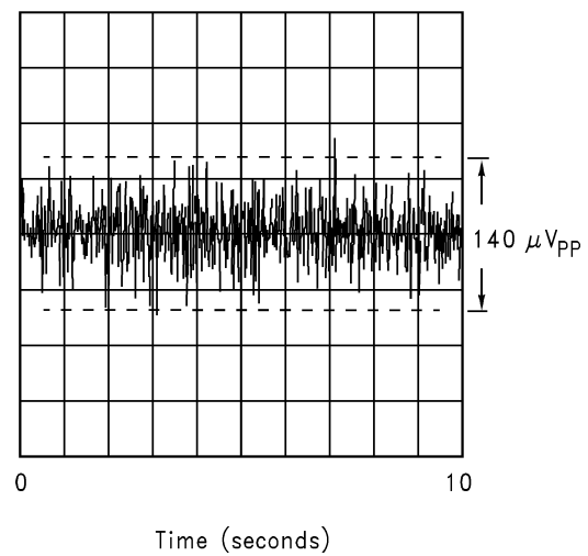
0.1Hz to 10 Hz Noise ( V_{REF} = 2.5\text{V} )
