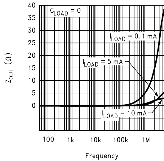
Output Impedance
