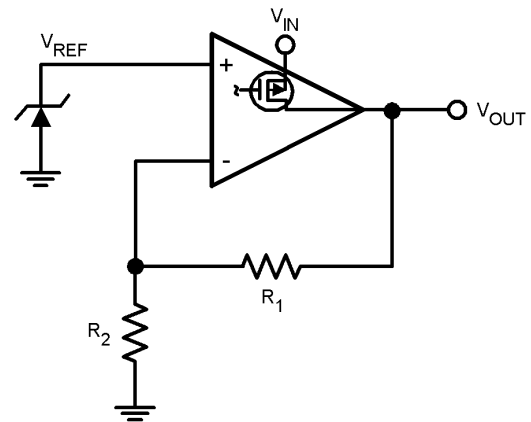
FIGURE 3. Regulator Topology Simplified
