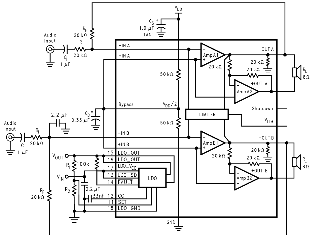
FIGURE 1. Typical Audio Amplifier Application Circuit Pin out shown for the LLP package. Refer to the Connection Diagrams for the pinout of the TSSOP package.
