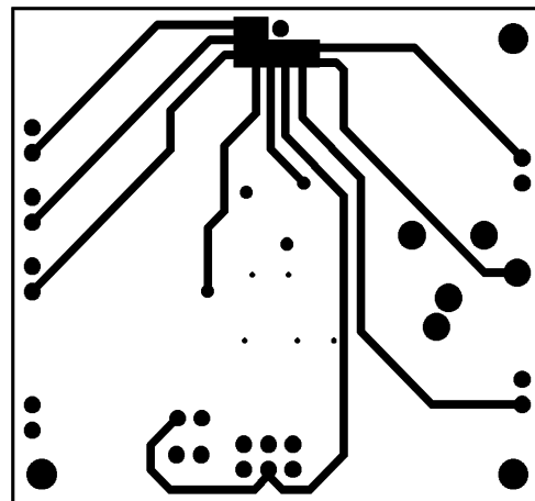
Recommended ITL PC Board Layout: Middle 2 Layer
