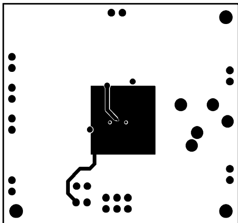
Recommended ITL PC Board Layout: Middle 1 Layer
