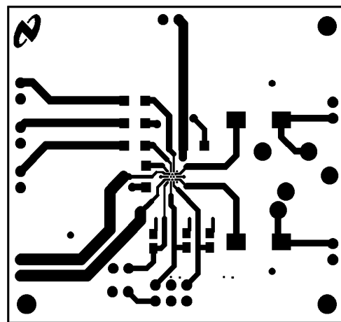
Recommended ITL PC Board Layout: Top Layer
