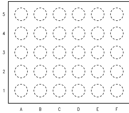
30 Bump ITL Package
