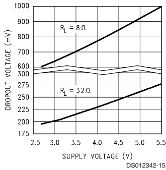
Dropout Voltage vs Power Supply
