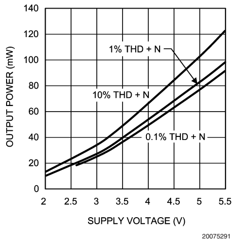
Output Power vs Supply Voltage R_L = 32\Omega , f = 1kHz
