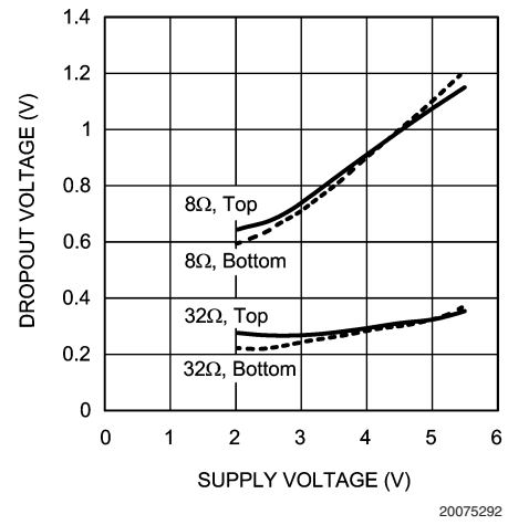
Clipping Voltage vs Supply Voltage
