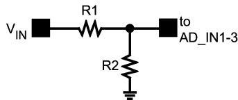
Required External Scaling Resistors for +12V Power Input
