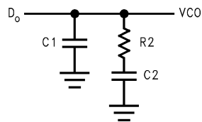
FIGURE 3. Passive Loop Filter
