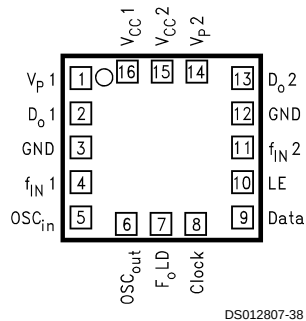
LMX2335L (Top View)
