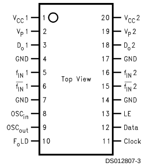
LMX2336L (Top View)
