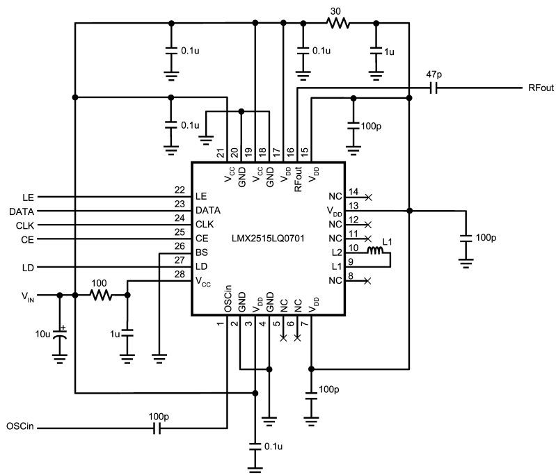
LMX2515LQ0701 Application Circuit
