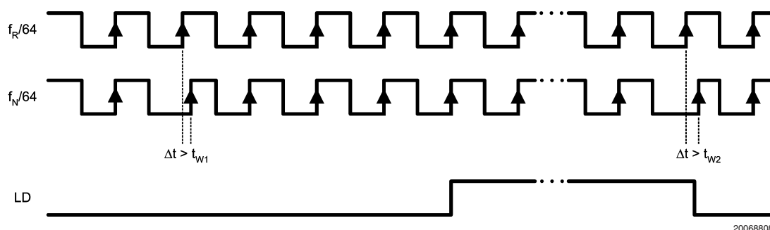
FIGURE 2. Lock Detect Timing Diagram Waveform (Notes 9, 10, 11, 12, 13)
