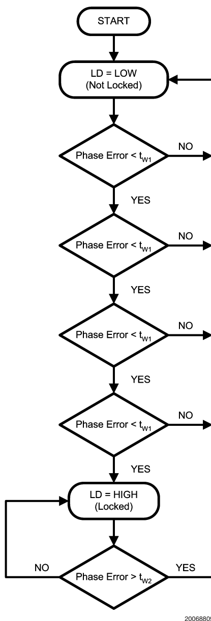
FIGURE 3. Lock Detect Flow Diagram
