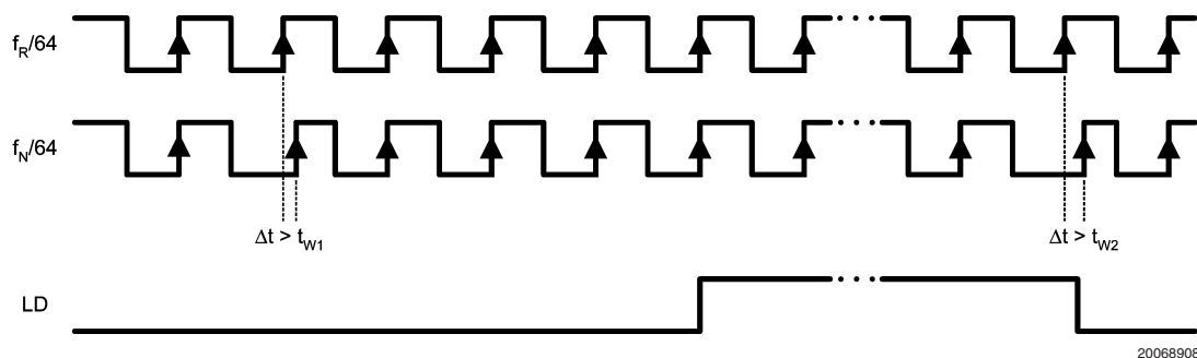
FIGURE 2. Lock Detect Timing Diagram Waveform (Notes 12, 13, 14, 15, 16)
