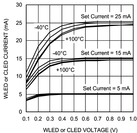
WLED or CLED Output Current vs Voltage Temperatures -40^{\circ}\text{C} , 25^{\circ}\text{C} , 85^{\circ}\text{C} , 100^{\circ}\text{C}
