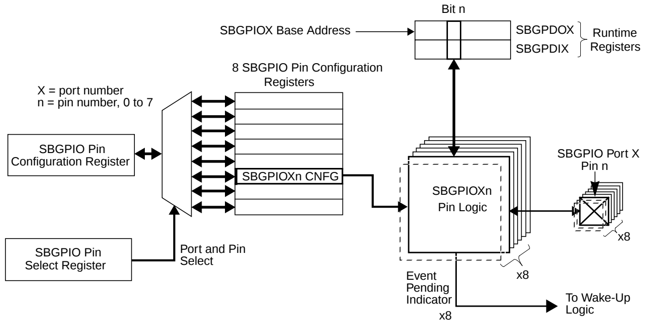
Figure 10. SBGPIO Port Architecture
