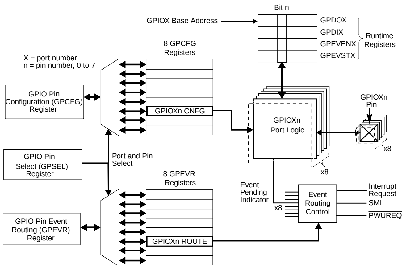
Figure 17. GPIO Port Architecture
