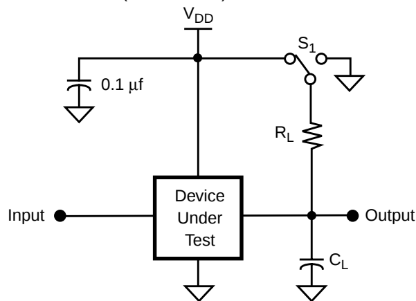
Figure 37. AC Test Conditions, T_A = 0^\circ\text{C} to 70^\circ\text{C} , V_{DD} = 5.0\text{V} \pm 10\%
