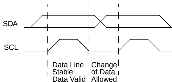
Figure 22. Bit Transfer
