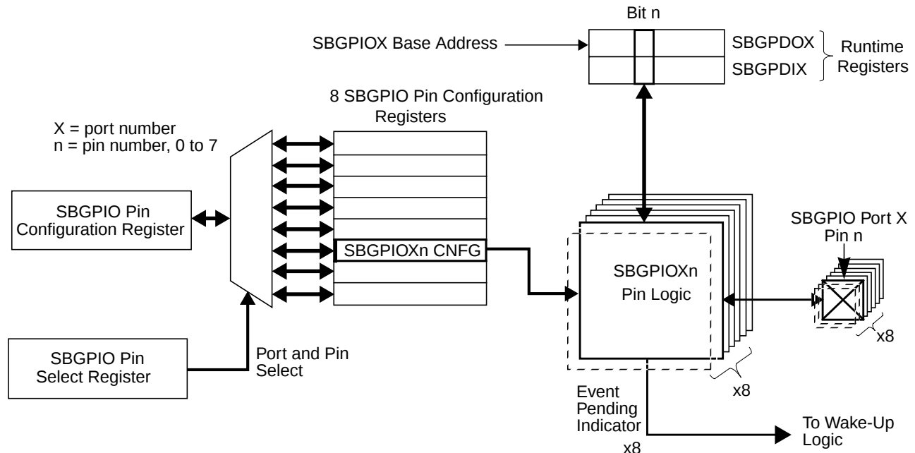
Figure 11. SBGPIO Port Architecture
