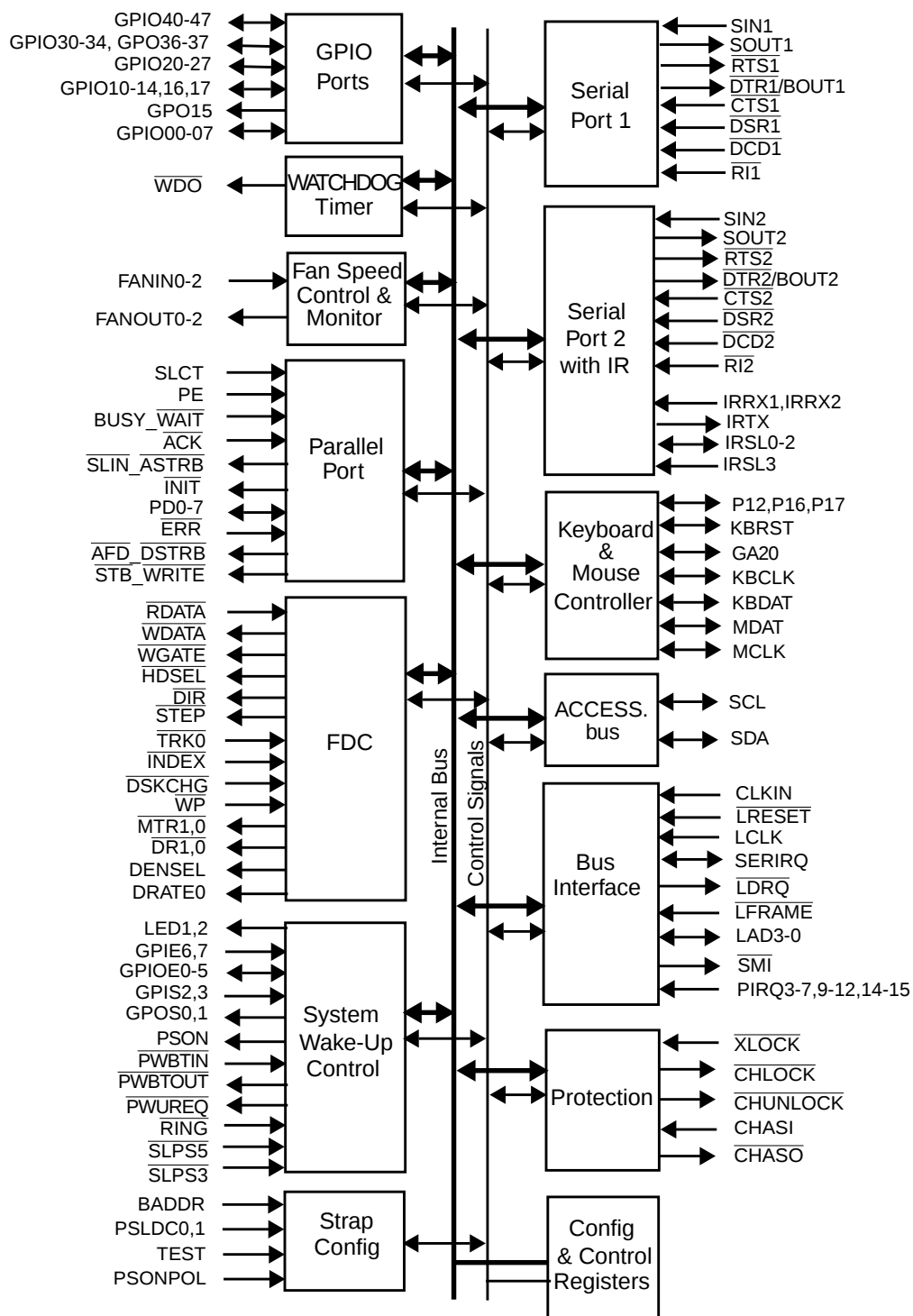
Figure 1. PC87364 Detailed Block Diagram
