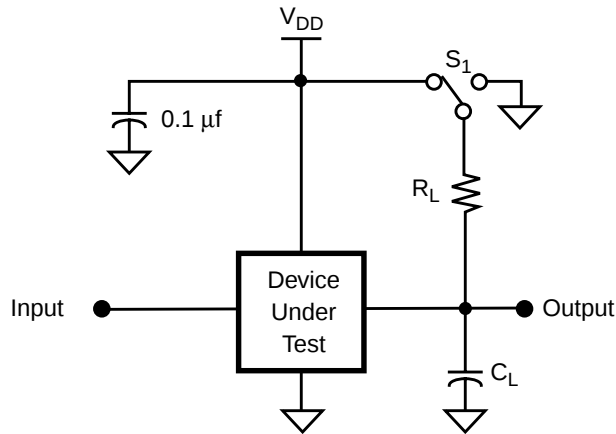
Figure 30. AC Test Conditions, T_A = 0^\circ\text{C} to 70^\circ\text{C} , V_{DD} = 5.0\text{V} \pm 10\%
