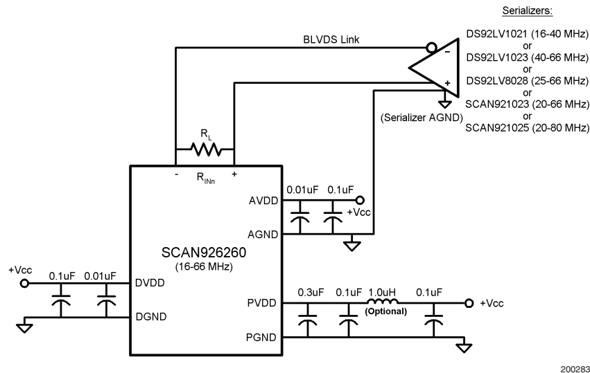
FIGURE 10. Typical Application Circuit (Only one power/ground for each supply type shown for clarity-bypass networks should be repeated for all power/ground pairs.)
