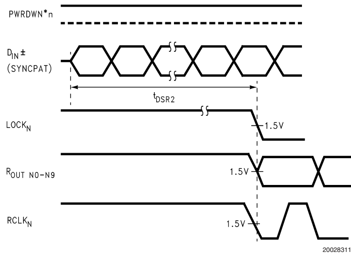
FIGURE 5. Locktime to SYNCPT t_{\text{DSR2}}
