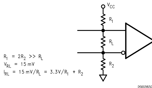
FIGURE 11. Optional Additional External Failsafe Biasing
