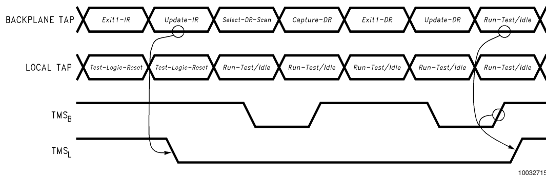
FIGURE 11. Local Scan Port Synchronization on Second Pass
