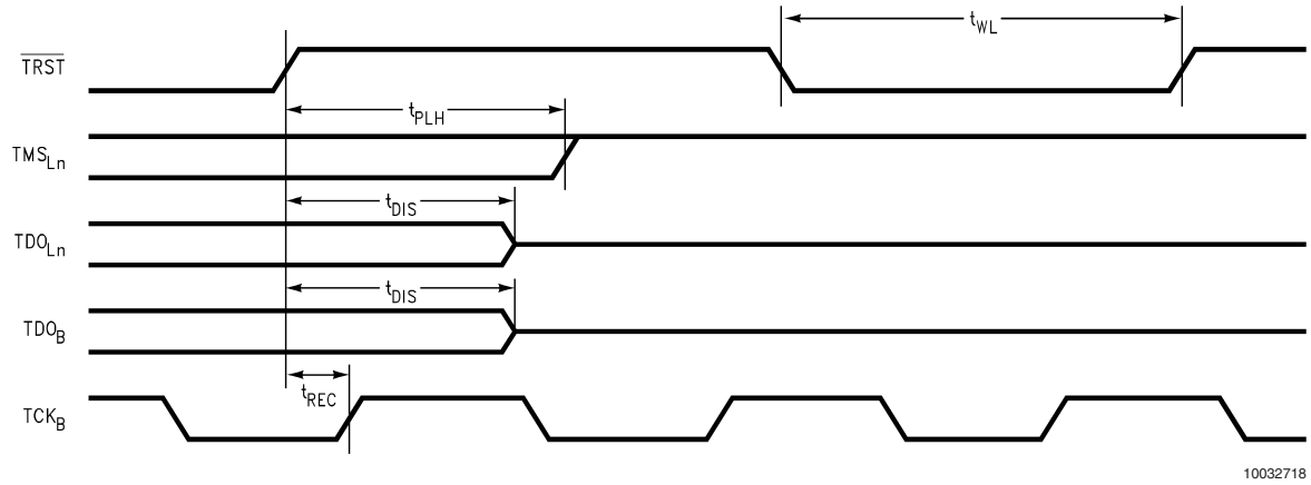
FIGURE 15. Reset Waveforms
