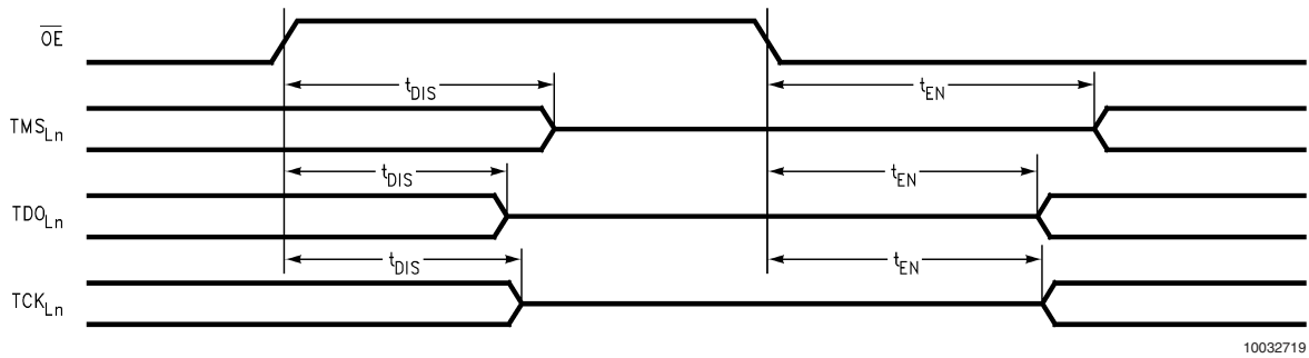
FIGURE 16. Output Enable Waveforms
