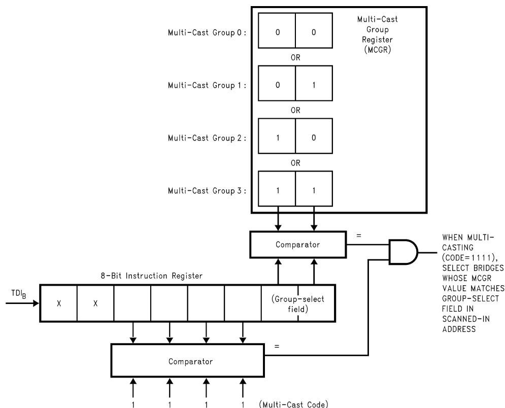
FIGURE 8. Multi-Cast Addressing: Address Loaded into Instruction Register
