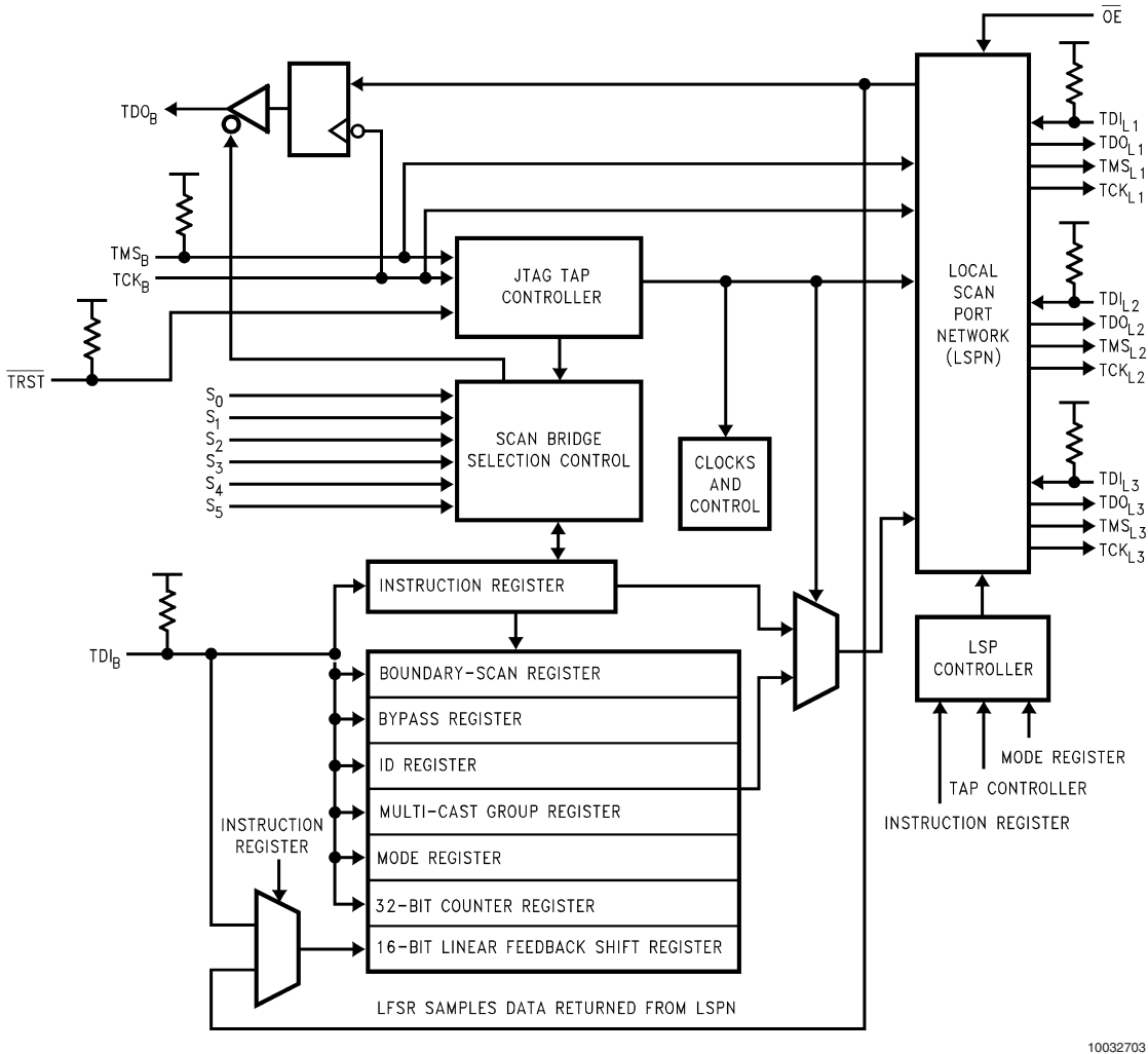
FIGURE 1. SCANPSC110F Bridge Architecture
