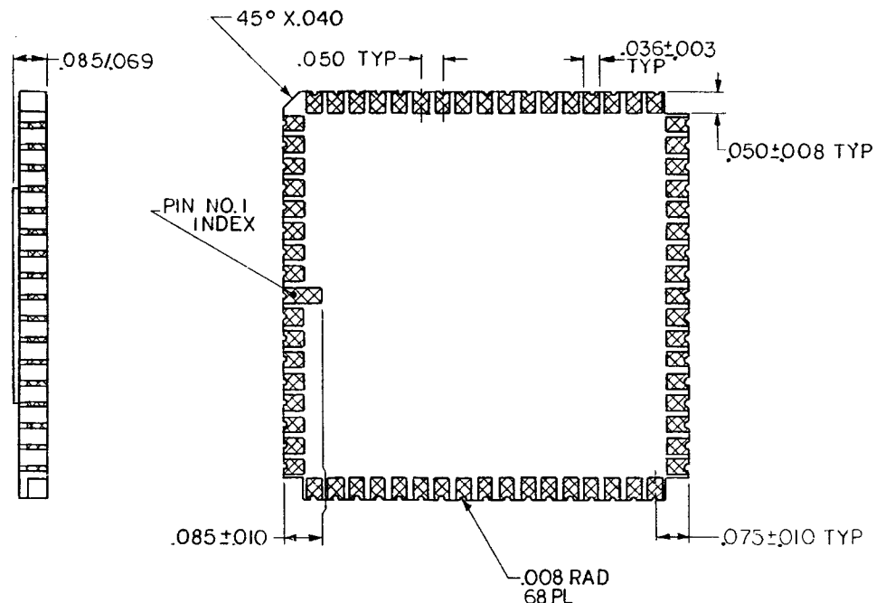
SIDE VIEW
