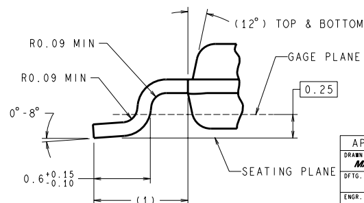
DETAIL A TYPICAL, SCALE: 40X
