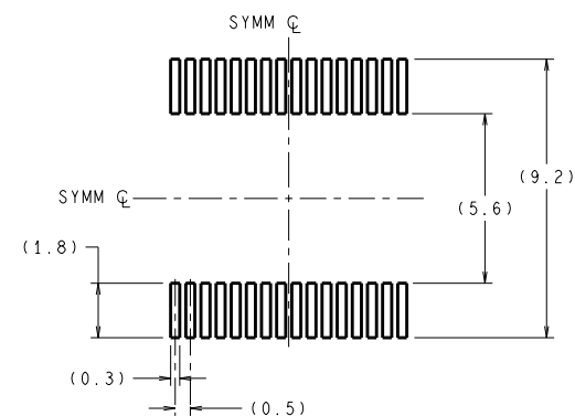
LAND PATTERN RECOMENDATION
