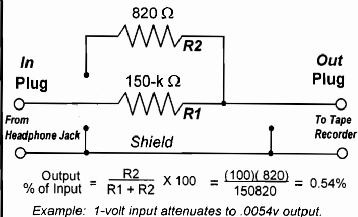
FIGURE 7: AUDIO DUBBING ADAPTER
