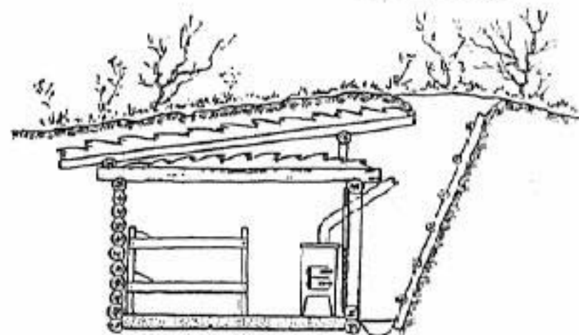
Picture 21a. Earthbunker (cutaway)
