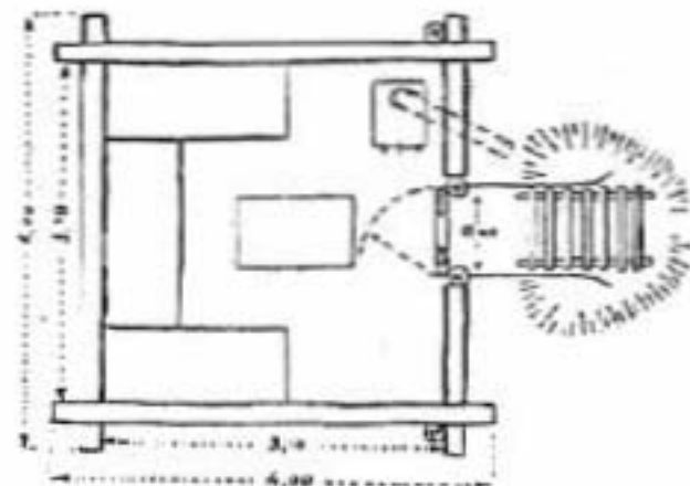
Picture 21b. Earthbunker (Layout)
