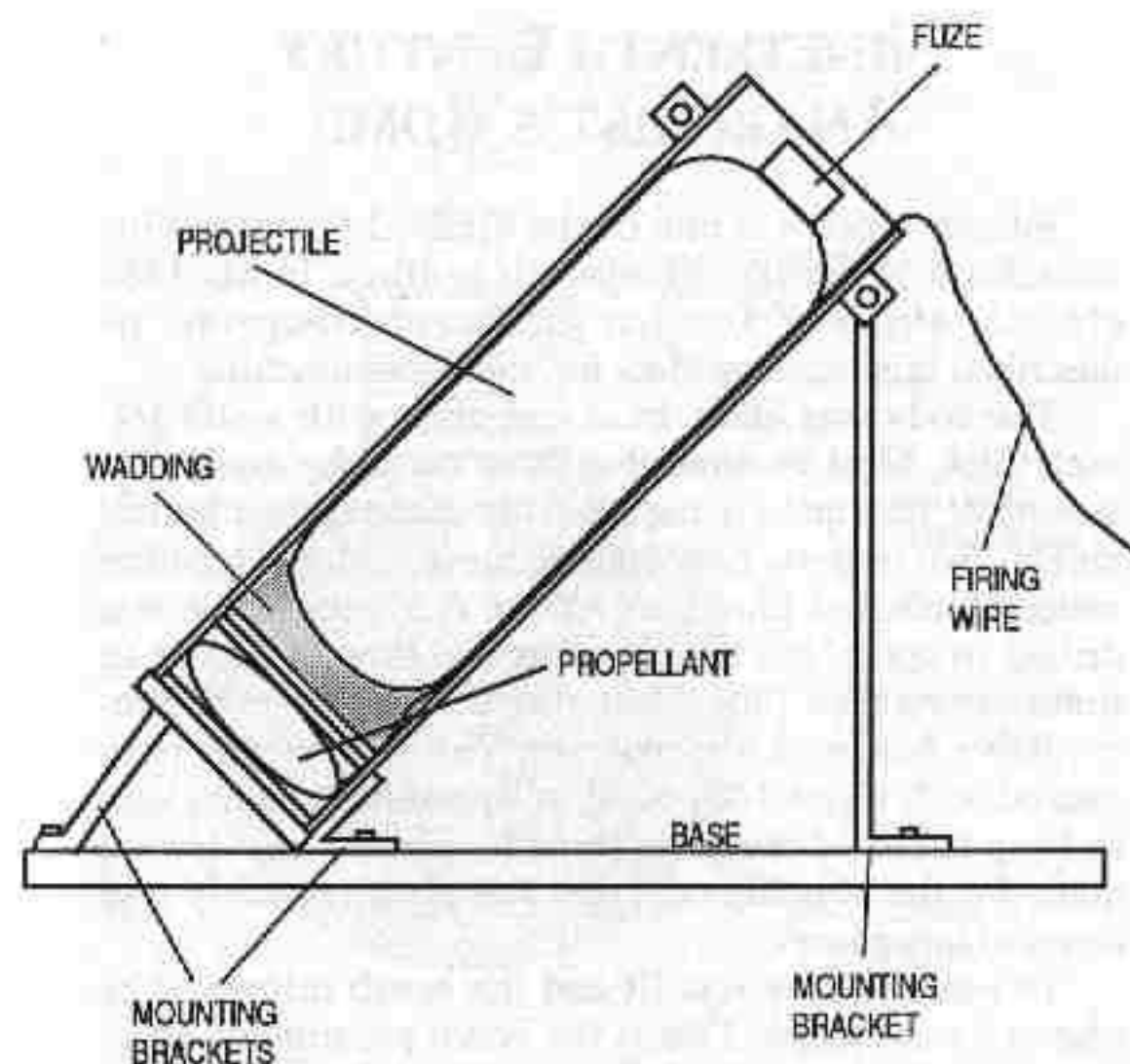
Sectioned view of IRA truck mortar.
