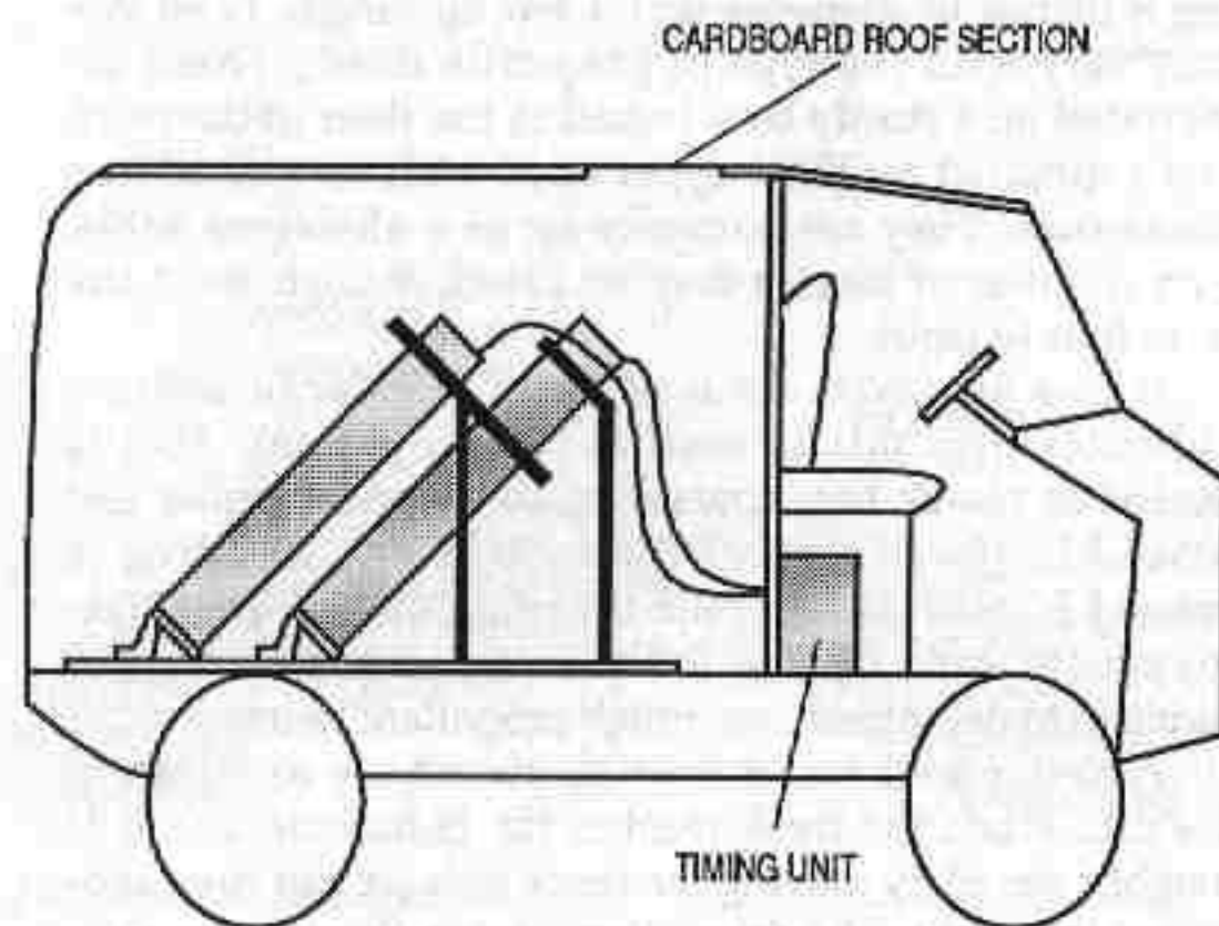
IRA truck mortar mounting.
