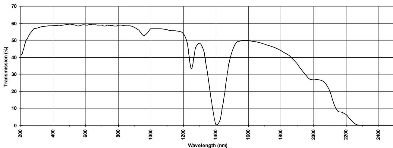
Spectral Transmission for 1 M Bundle, Fiber Type UV-QQ
