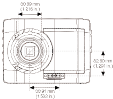
Figure 2. Camera Front
