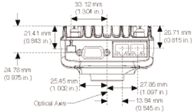
Figure 5. Camera Bottom
