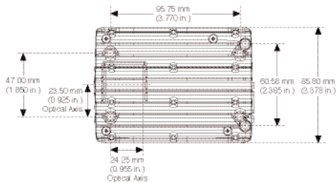
Figure 3. Camera Back
