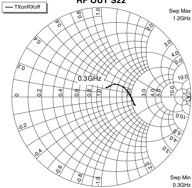
RF OUT S22
