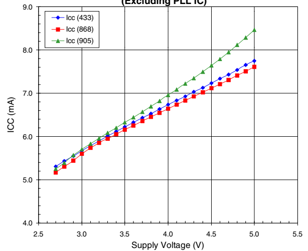
Receive Current versus V_{CC} (Excluding PLL IC)
