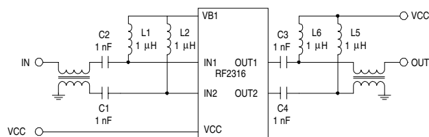
Figure 14. External connections for the RF2316
