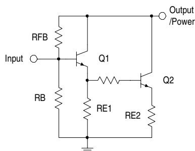
Figure 9. Darlington gain block
