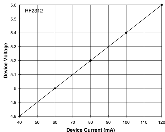
Figure 10. Device voltage vs. device current
