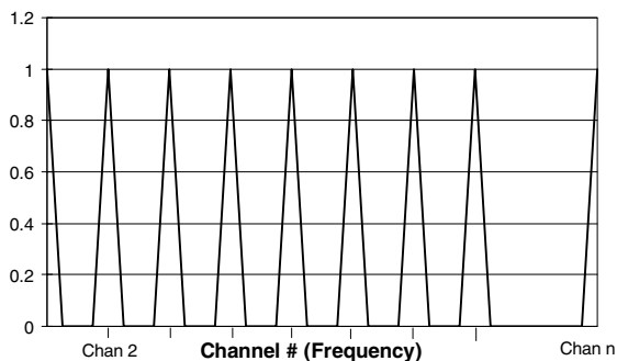
Figure 1. CATV Spectrum
