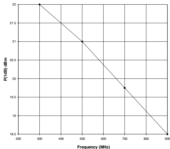
Figure 12. P1dB vs. frequency
