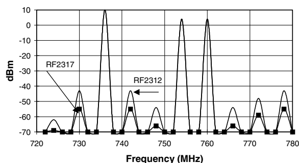
Figure 6. IM distortion with Three-Tone Input
