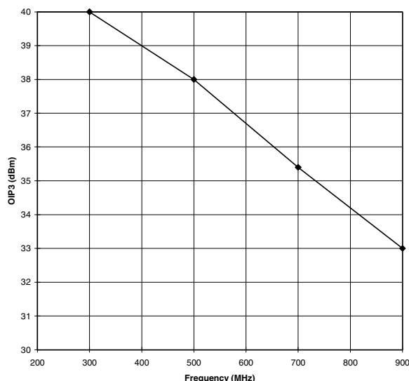
Figure 11. OIP3 vs. frequency
