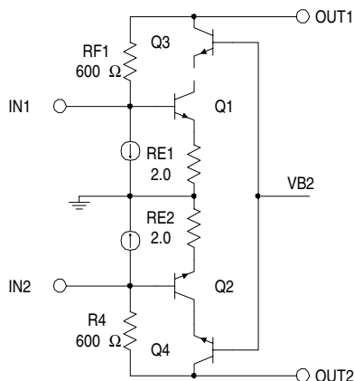
Figure 13. Cascode push-pull amplifier
