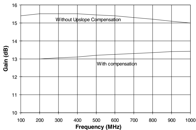
Figure 15. Gain vs. frequency
