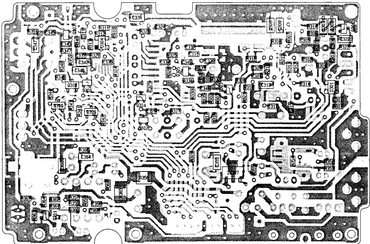
Bottom View
