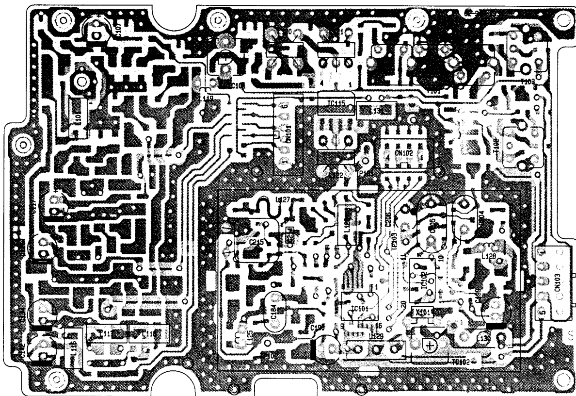
Top View
