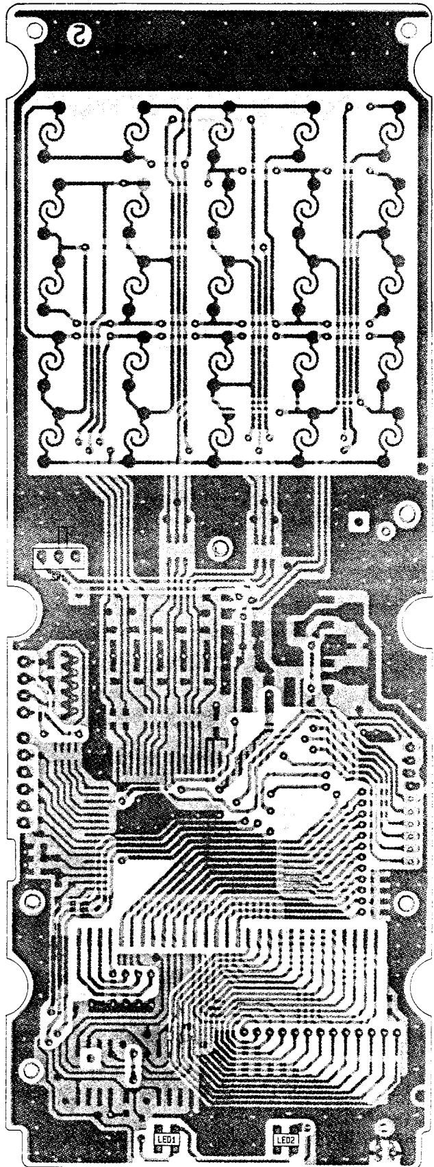
Bottom View
