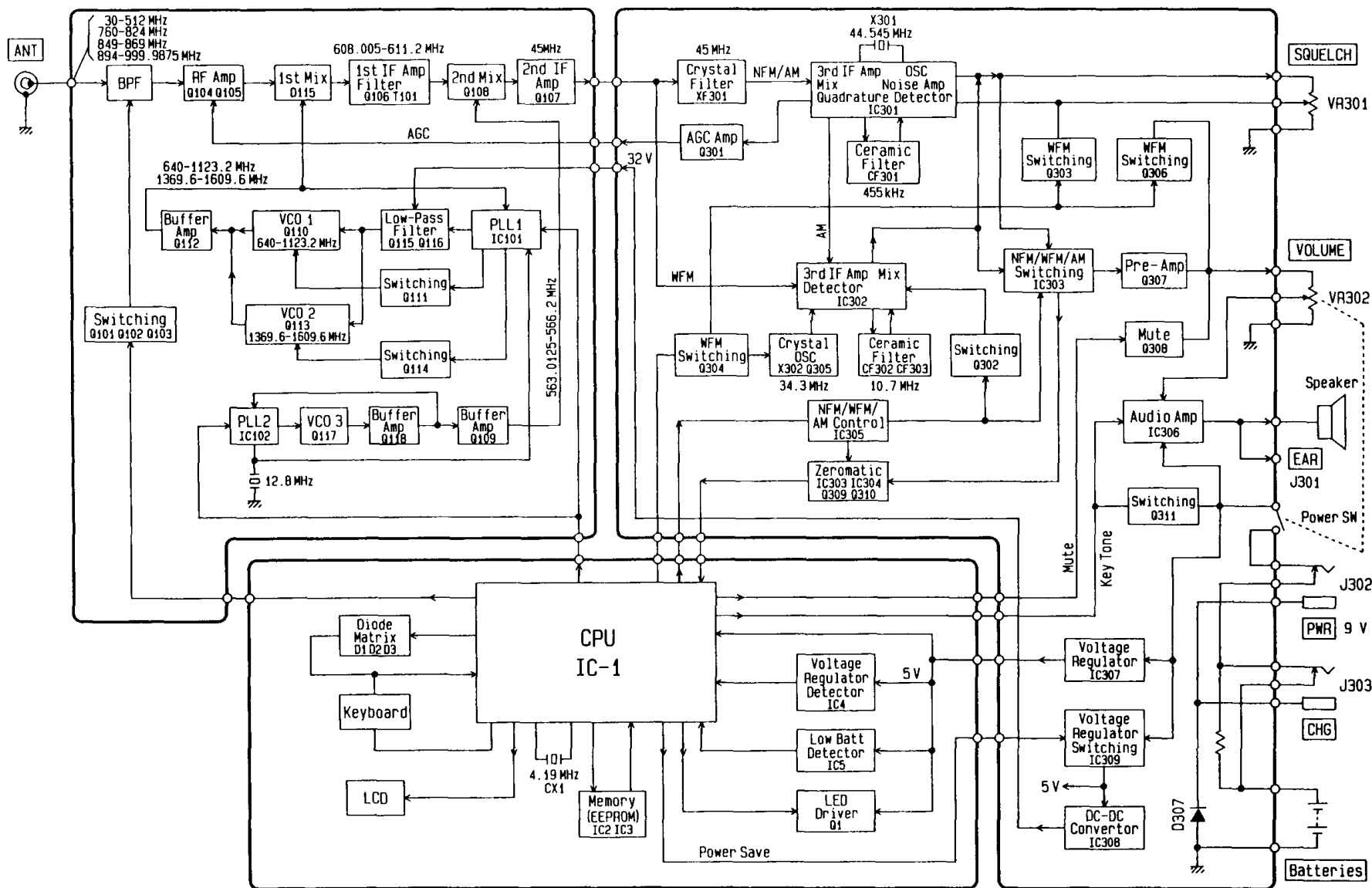
BLOCK DIAGRAM
