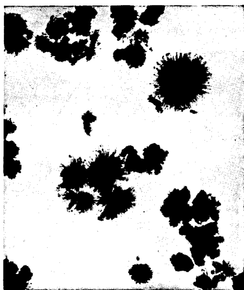
GALACTOSAZONE
