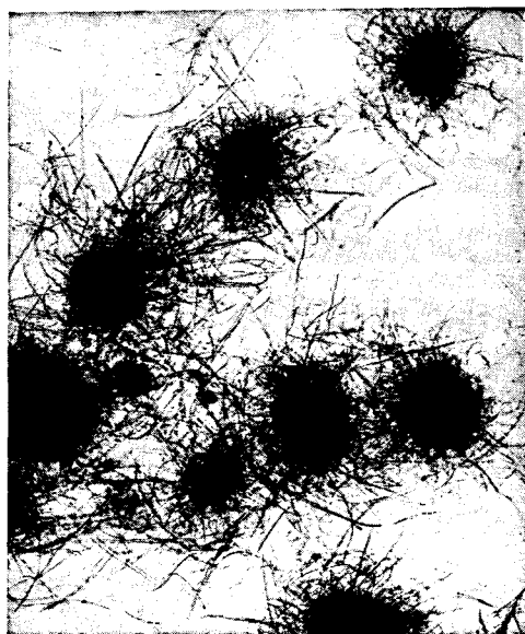
LACTOSAZONE
