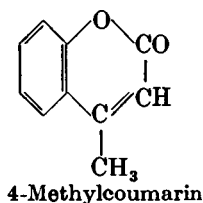
4-Methylcoumarin
