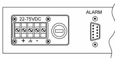
Figure 2 DC Power Connection
