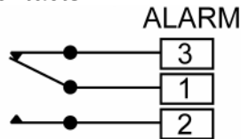
Figure 5. Alarm Contacts
