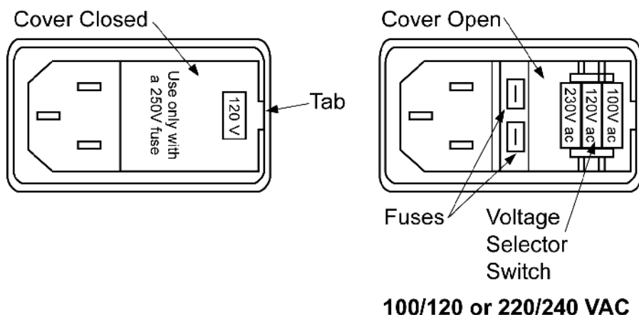
Figure 1 AC Input Filter/Fuses/Voltage Selector
