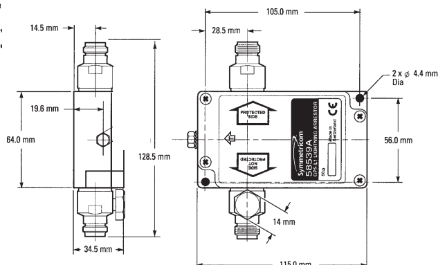
58539A GPS L1 Lightning Arrestor Dimensions
