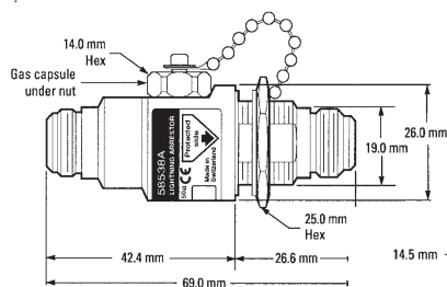
58538A Lightning Arrestor Dimensions
