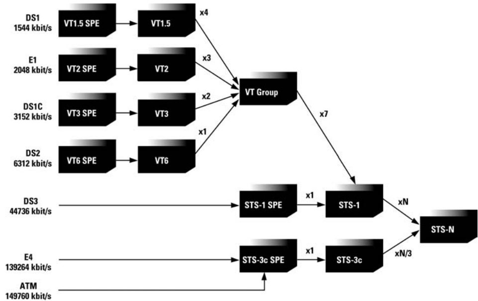
Figure 2. SONET Multiplexing
