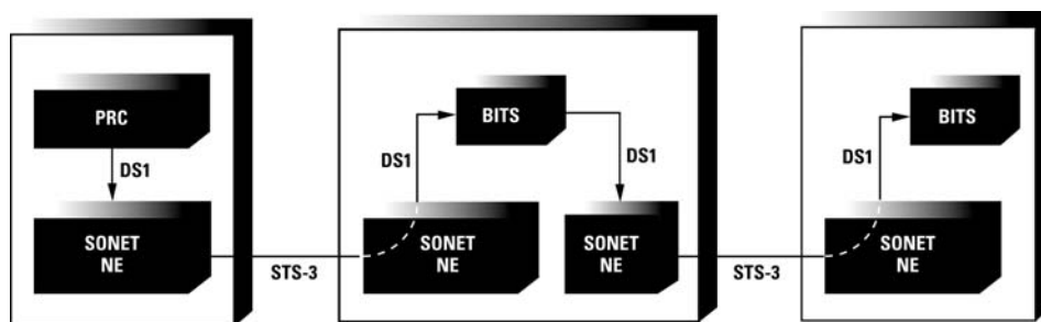
Figure 9. Typical SONET network synchronization plan
