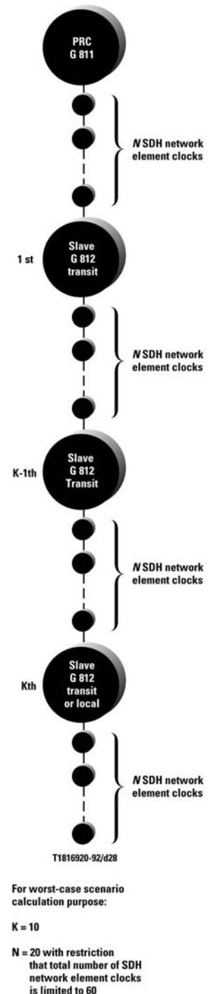
Figure 7. SDH synchronization network reference chain
