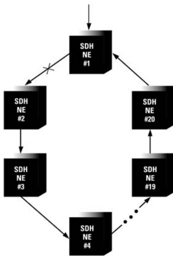
Figure 8a. SDH ring with a normal timing flow counterclockwise
