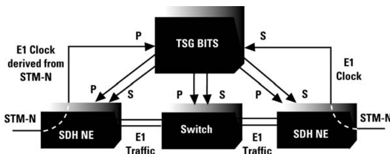
Figure 5. Timing distribution using SDH lines
