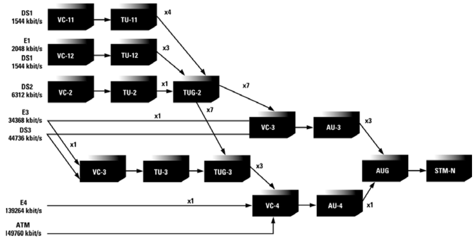
Figure 1. SDH Multiplexing
