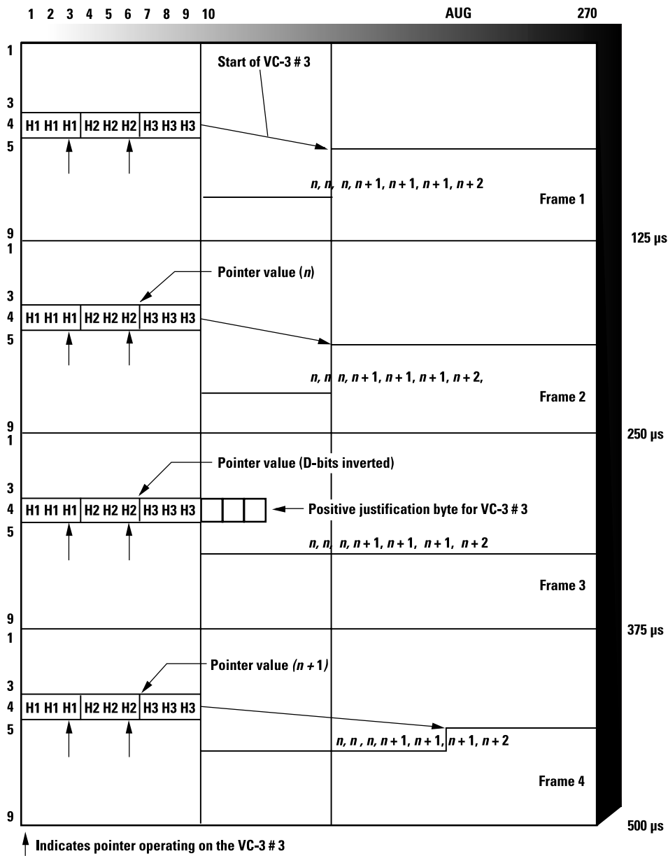
Figure 4. AU-3 pointer adjustment operation—positive justification
