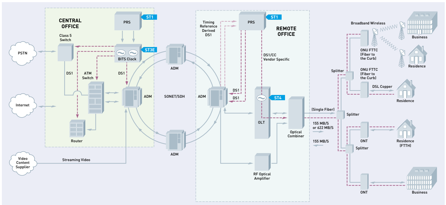
FIG.4 The Stratum 1 clock source is transported over SONEt to the BITS clock in Office "B" where the OLT is located. A network failure or rearrangement that results in the BITS clock in Office "B" losing its Stratum 1 reference will result in the BITS clock entering holdover at the Stratum 3 level, which meets compliance to the G.983.1 recommendations.
