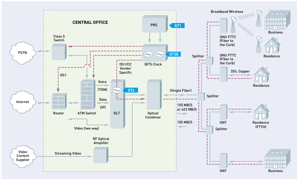
FIG.5 This illustration shows the BITS clock co-located in the same facility as the PRS Stratum 1 source and the OLT. A failure of the PRS would result in the BITS clock entering holdover and providing the required clock accuracy for all office elements including the OLT until the PRS can be restored.
