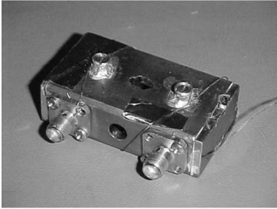
Figure 7: 9.2 GHz RF resonance cavity
