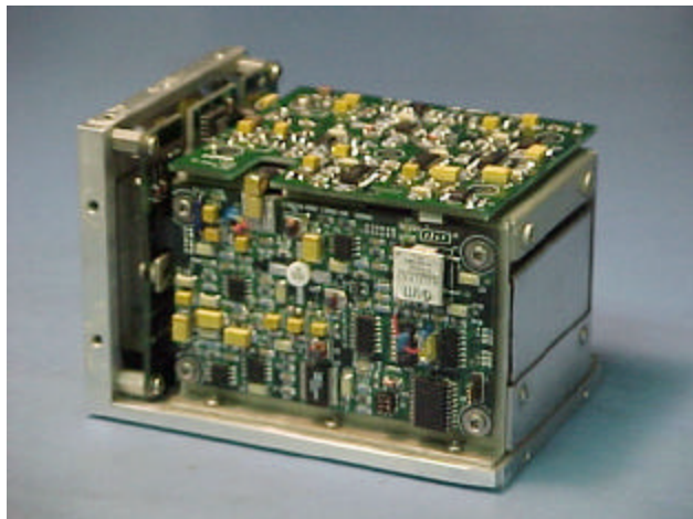
Figure 6 – Main Assembly
