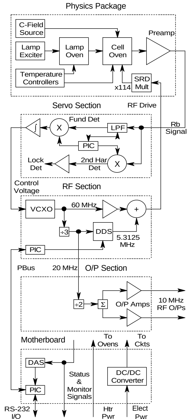
Figure 4 – Block Diagram
