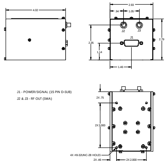
Figure 2 – Mechanical Interface
