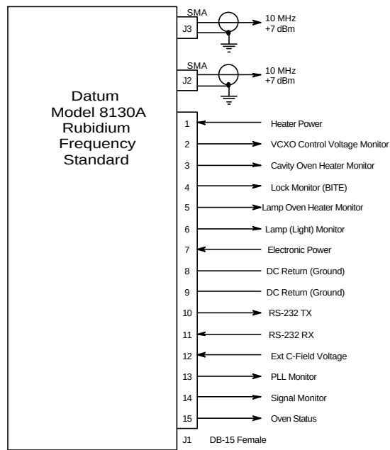
Figure 3 – 8130A Electrical Interface
