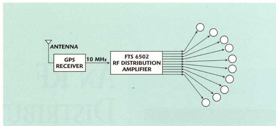
▲ Fig. 4 A GPS-derived signal distributed to multiple test stations.
