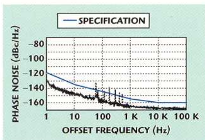
▲ Fig. 2 Measured phase noise at 4 MHz.
