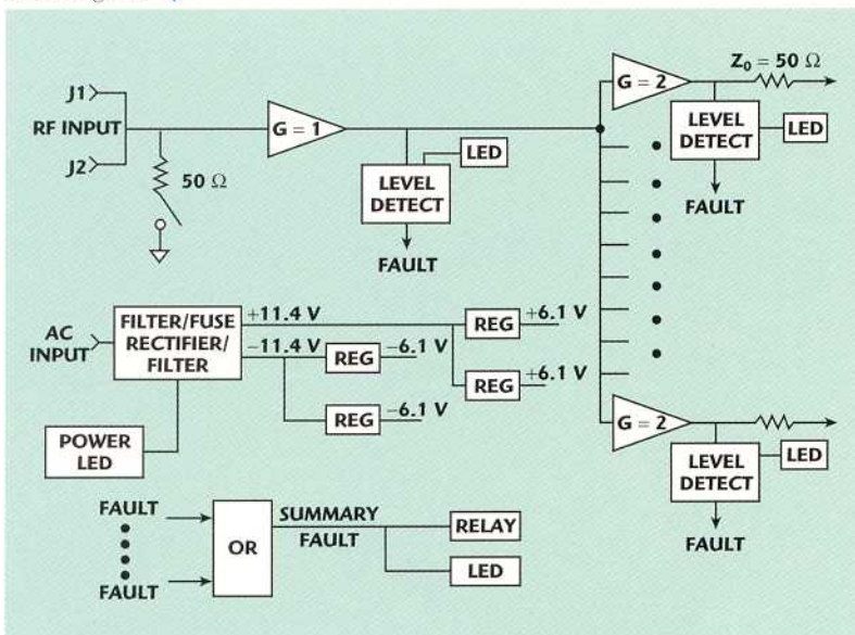
Fig. 1 The RF section's block diagram. ▼
