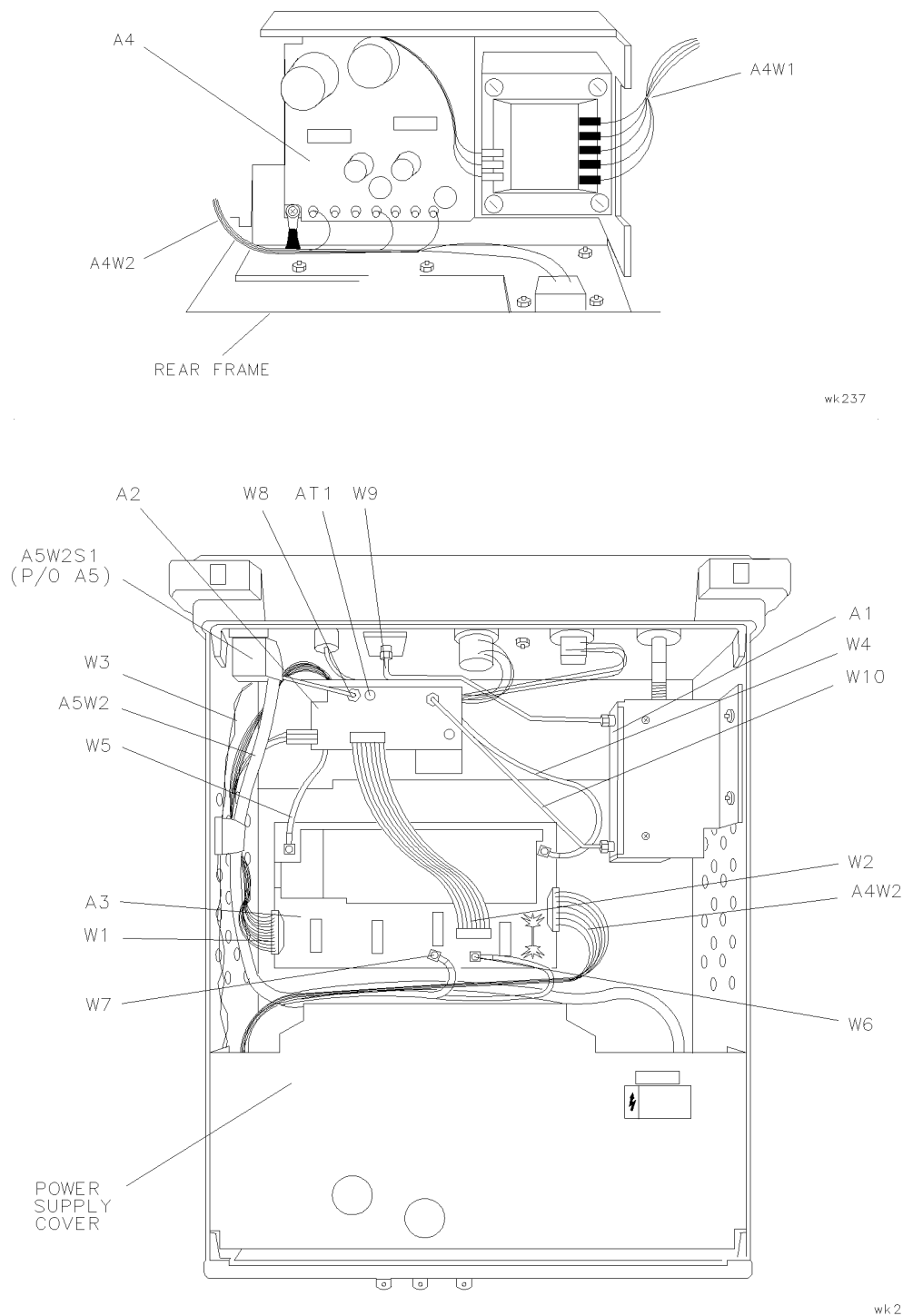
Figure 6-1. Major Assemblies and Cable Locations
