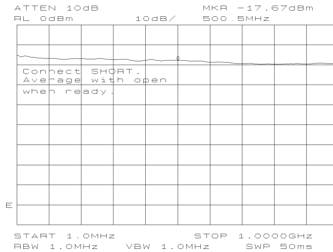
Figure 3-38. On-Screen Prompts to Connect a Short
