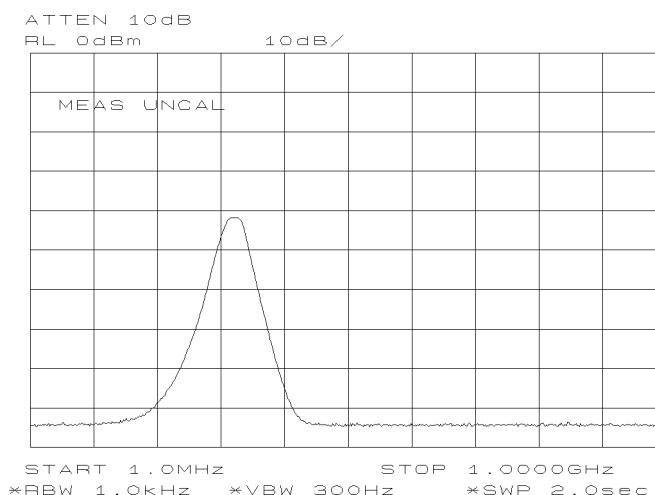
Figure 3-25. Decrease Resolution Bandwidth to Improve Sensitivity
