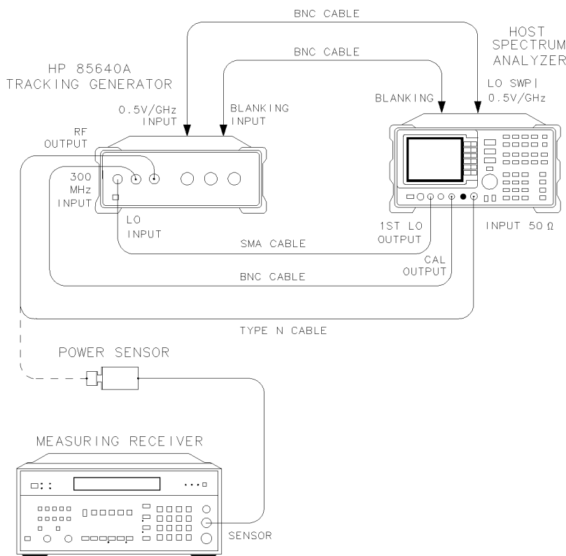
Figure 4-4. Level Flatness Test Setup
