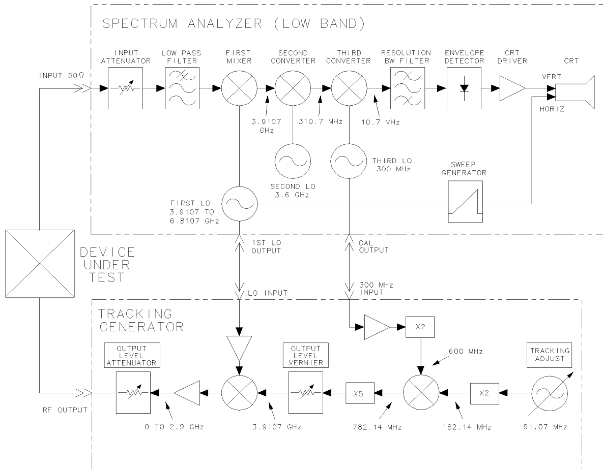
Figure 7-8. Simplified HP 85640A to Host Spectrum Analyzer System Block Diagram
