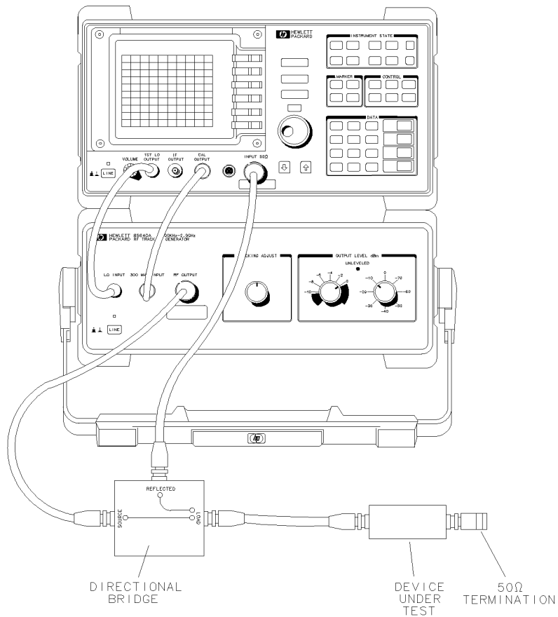
Figure 3-33. System Setup for a Reflection Measurement
