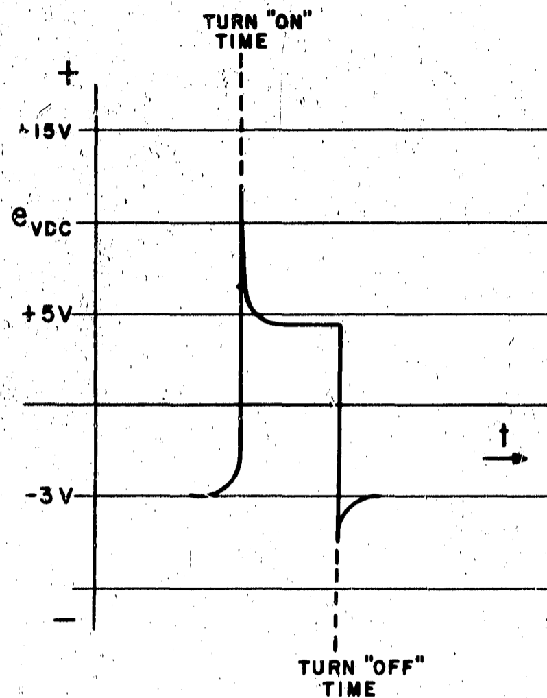
Figure 13. Dynamic Bias Switching Waveform
