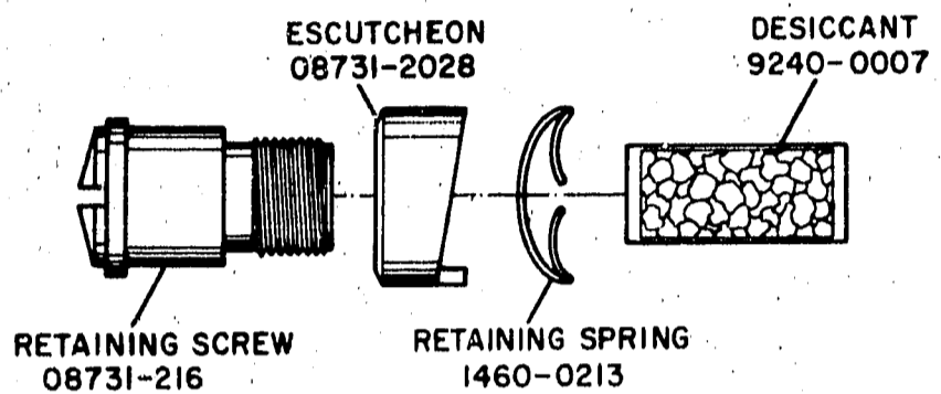
Figure 15. Dessicant Assembly
