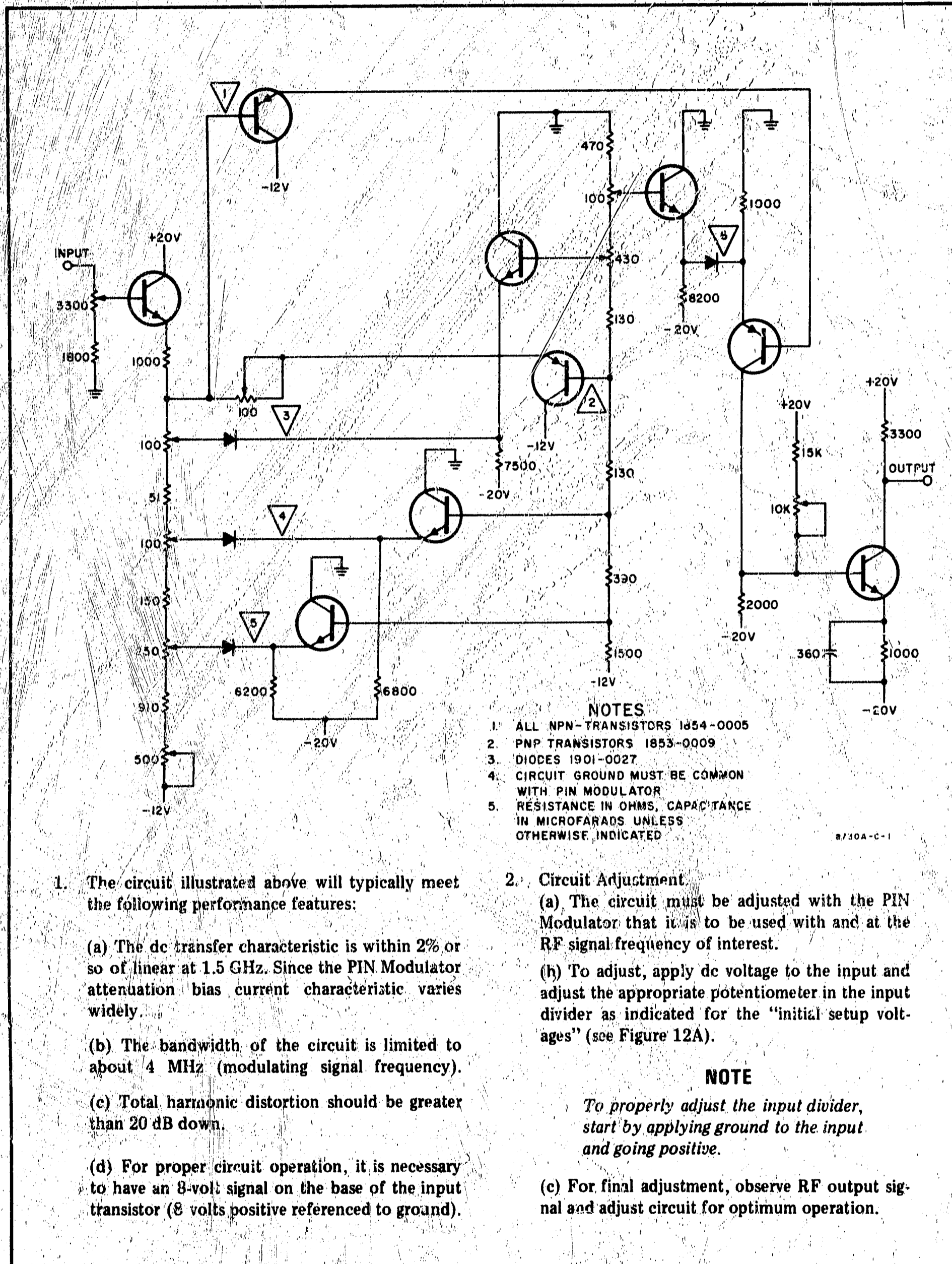
Figure 12B. Typical Shaping Circuit
