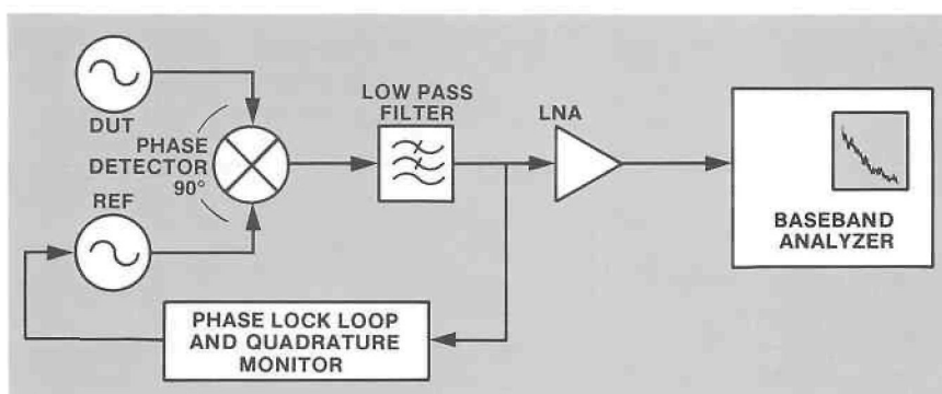
Figure 4. Basic Phase Detector Method implementation, using a double-balance mixer as the phase detector.
