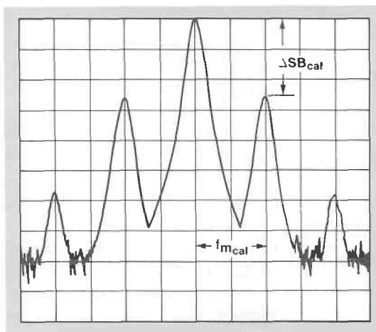
Figure 18. Carrier with a single FM tone used as the calibration signal.
