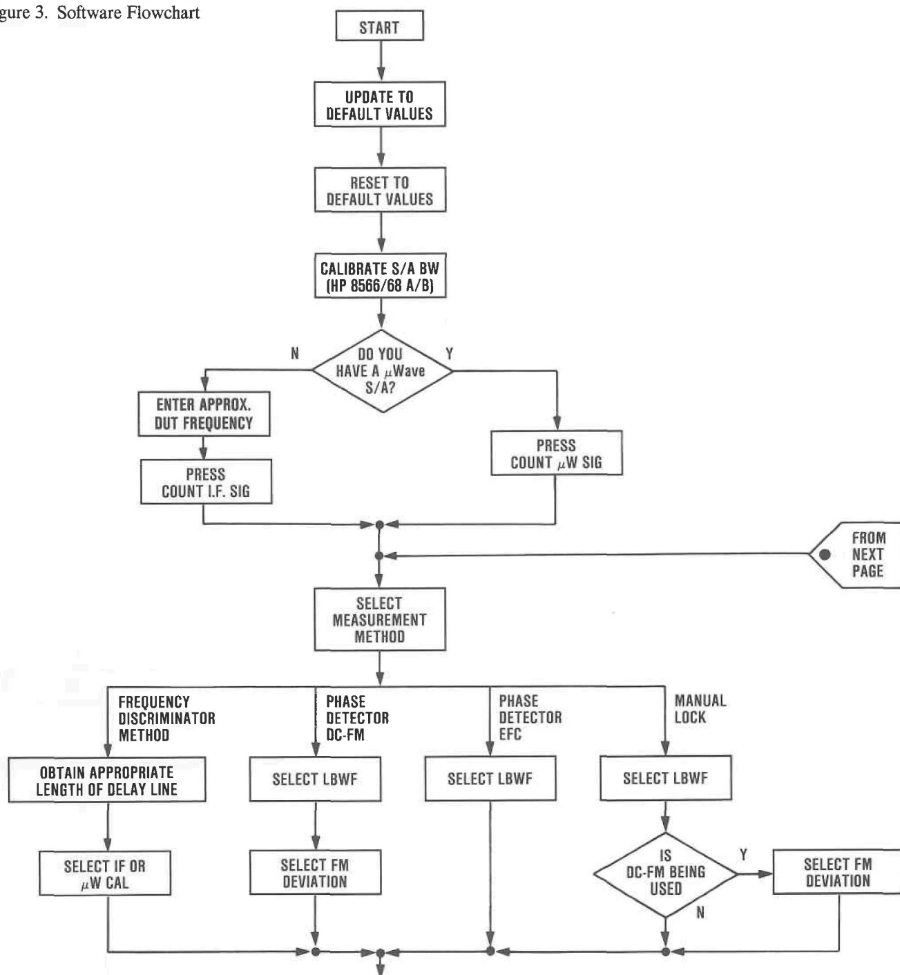
Figure 3. Software Flowchart
