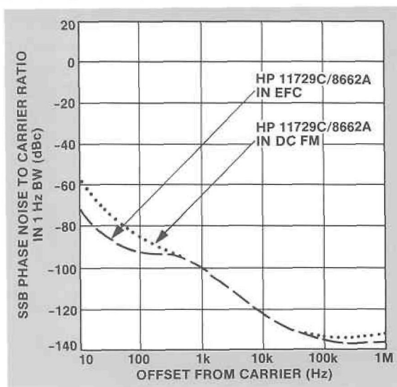
Figure 9. Typical system noise floor at 10 GHz using the Phase Detector Method.
