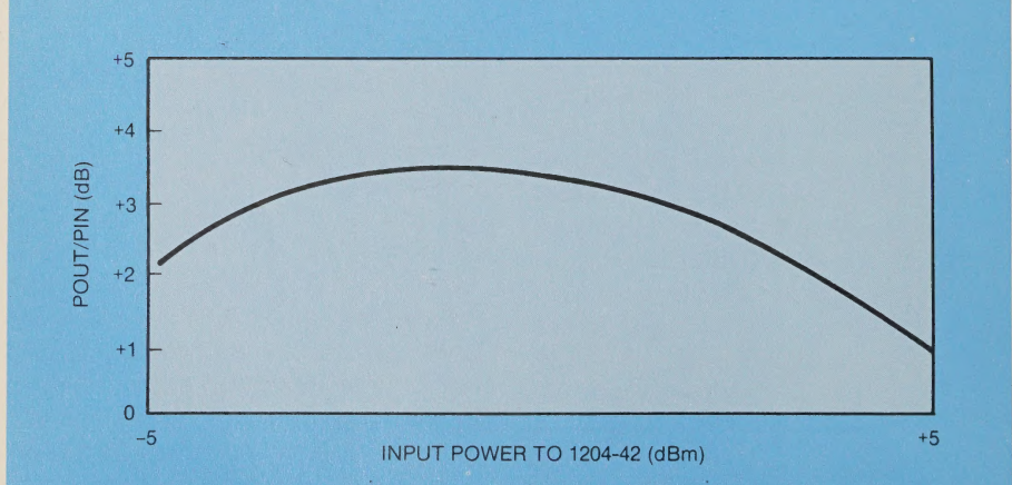
Figure 5B. Conversion efficiency at 50 GHz.
