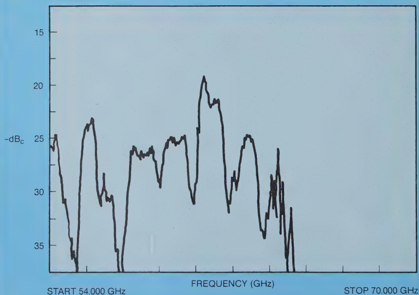
Figure 12. 40 to 60 GHz 4/3 f_0 harmonic.
