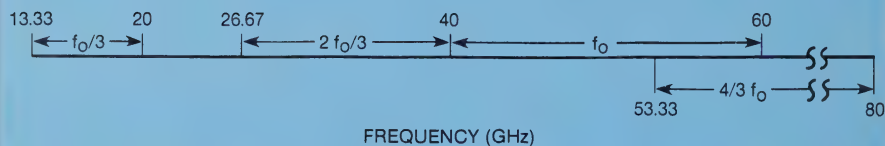
Figure 8B. 40 to 60 GHz harmonic products.
