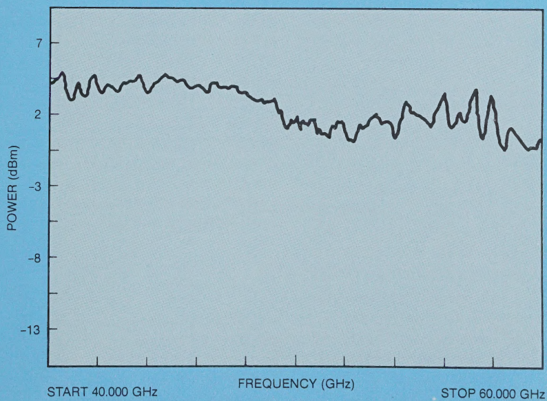
Figure 4B. Maximum output power.
