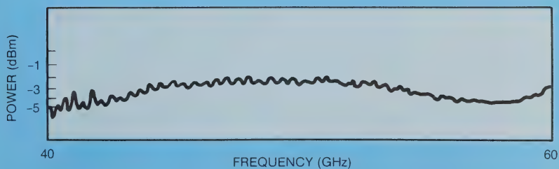
Figure 7. Externally leveled output power.
