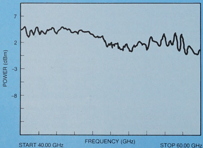
Figure 6. Maximum output power with externally leveled input power.
