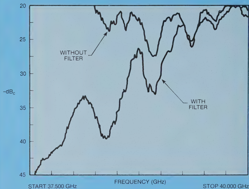
Figure 11. 40 to 60 GHz 2/3 f_0 harmonic with high-pass filter.
