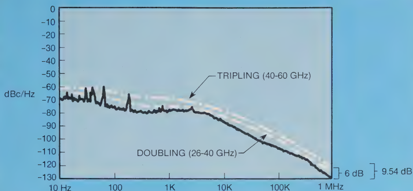
Figure 13. HP 8340A single-sideband phase noise.
