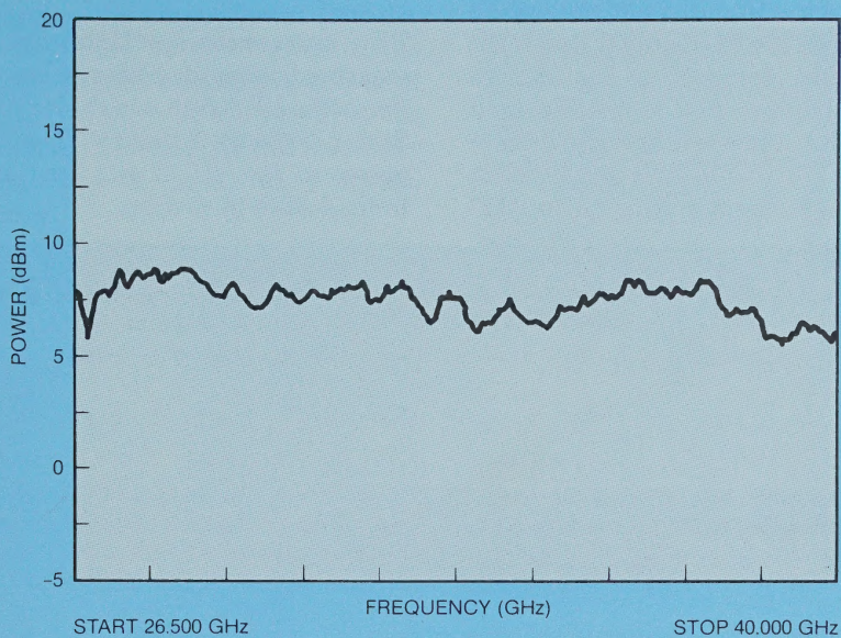
Figure 4A. Maximum output power.
