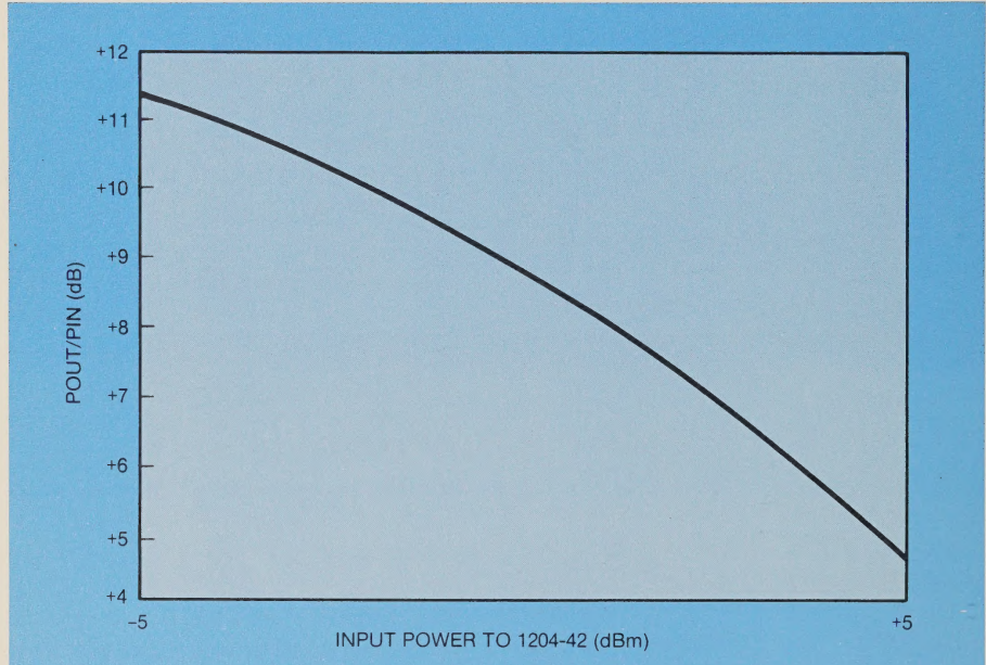
Figure 5A. Conversion efficiency at 33 GHz.
