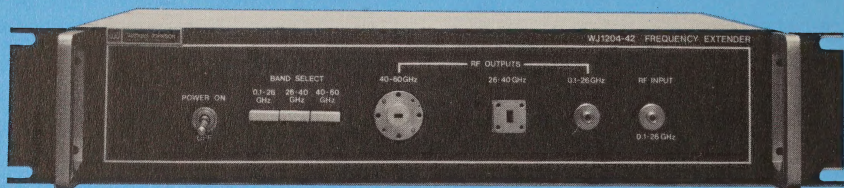
2 to 60 GHz signal source — HP8350/83595 and WJ-1204-42.
