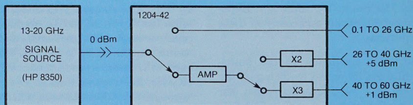
Figure 1. Frequency extender block diagram.
