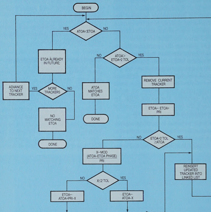
Figure 3. Time tracking algorithm.
