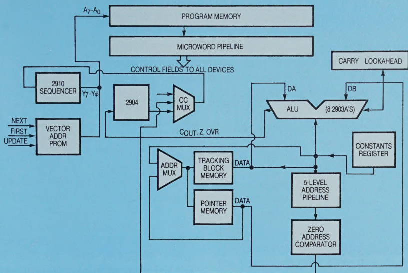
Figure 5. Time tracking processor block diagram.
