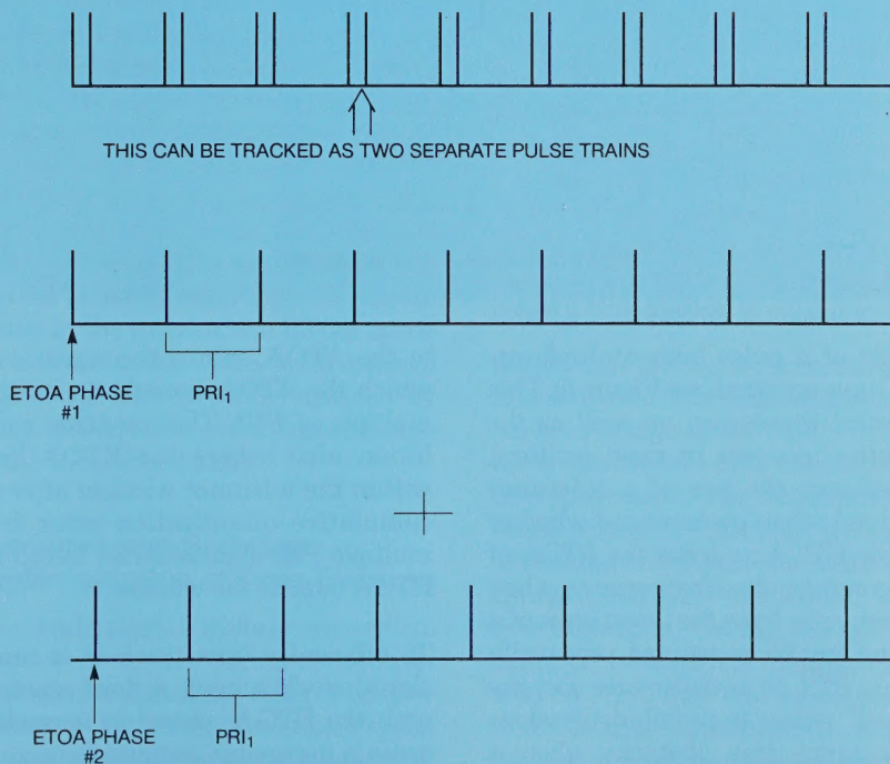
Figure 2. Time tracking of a two-position stagger.
