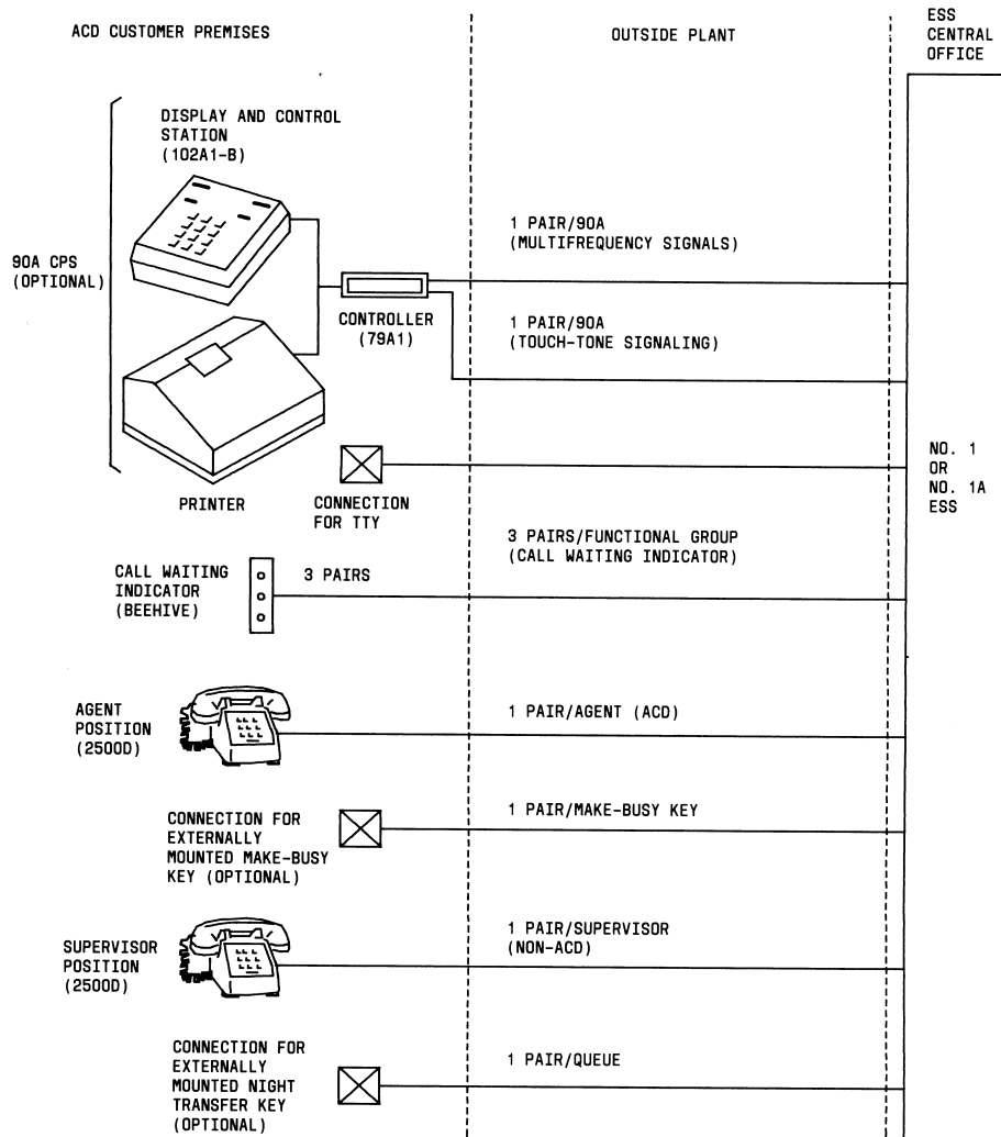
Fig. 1—Basic ACD Customer With Basic Telephone Sets
