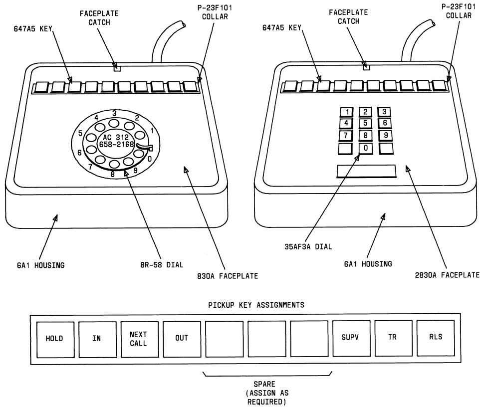
Fig. 4—Typical 10-Button Agent Telephone Sets
