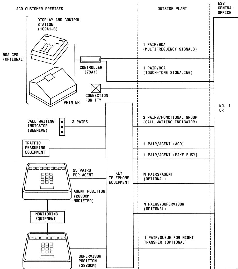
Fig. 3—Basic ACD Customer With 10-Button Key Telephone Sets
